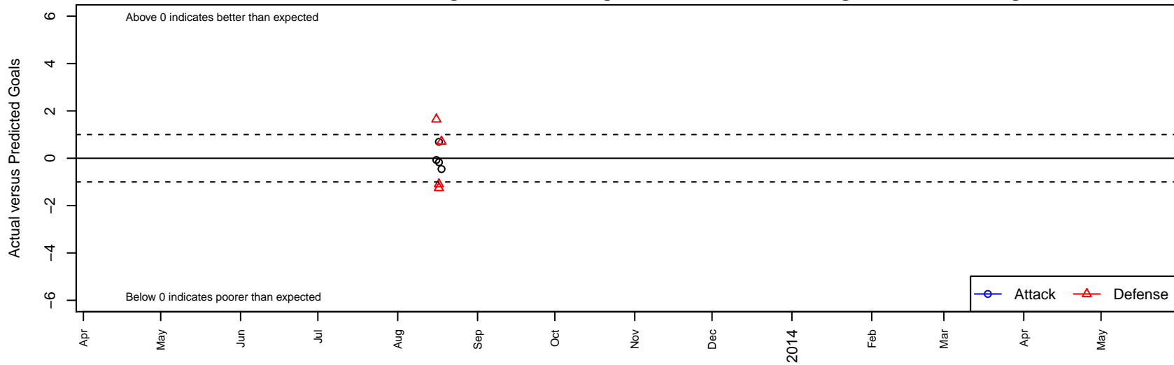
Storm FC B97 Dots are actual minus expected GF (blue circles) and GA (red triangles). Blue line is smoothed change in attack strength. Red is smoothed change in defense strength.
